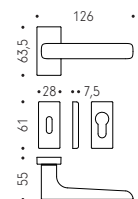
MR 11 RSM-RSMY Finishes: CR - CM
